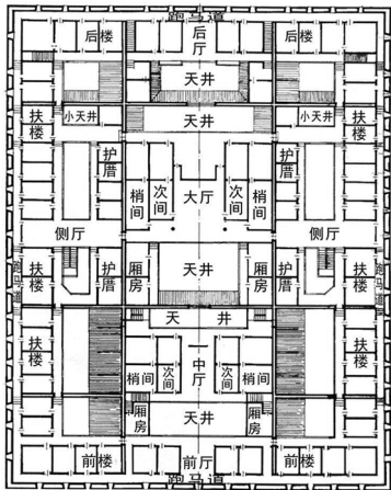
图 5 东关寨二层平面图 Fig.5 Plan of the second floor of Dongguan Walled Castle
