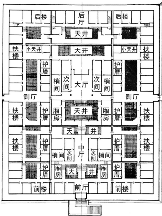
图 4 东关寨一层平面图 Fig.4 Plan of the first floor of Dongguan Walled Castle
